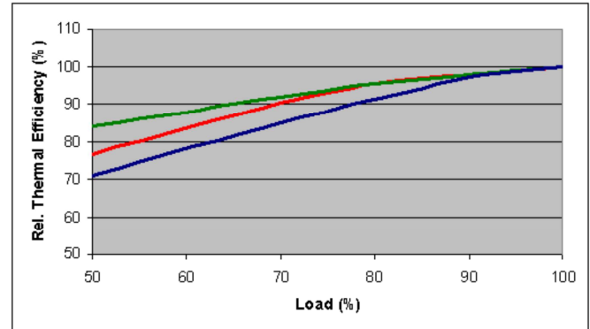
Figure 17. Thermal efficiency of typical industrial gas turbines as a function of load
