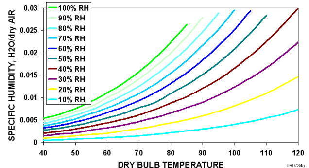
Figure 21. Graphic explanation of specific and relative humidity as a function of temperature
