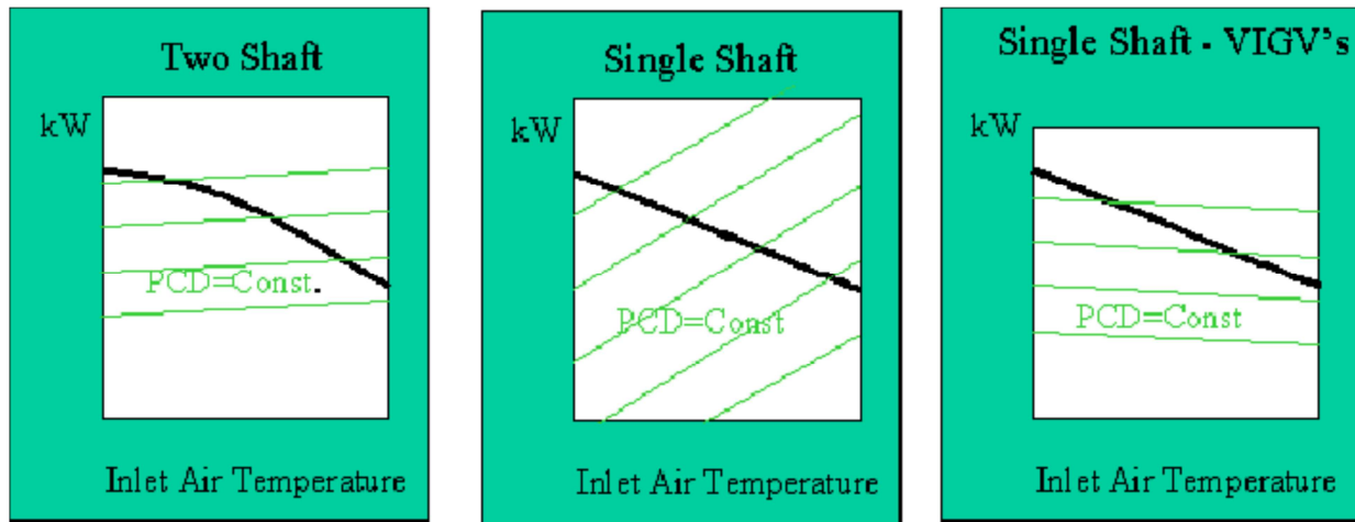
Figure 20. Effect of low fuel gas pressure on different engine designs. PCD is the pressure in the combustor.
