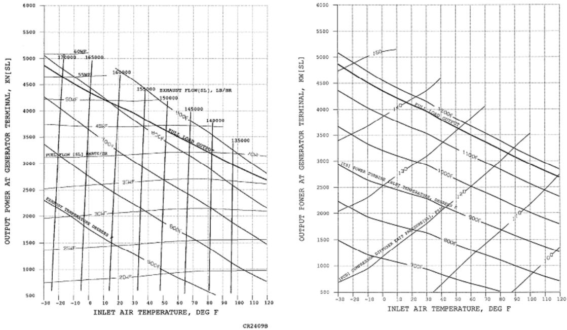
Figure 16. Single-shaft gas turbine performance map
