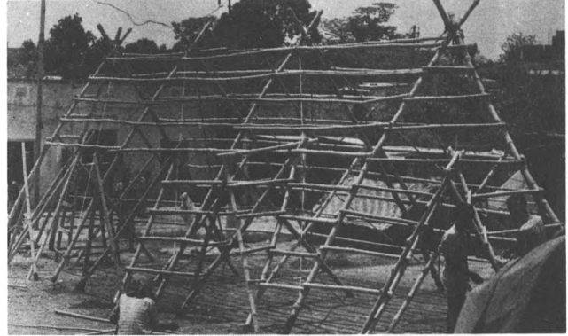
Figure 13. Diagonal Bracing
