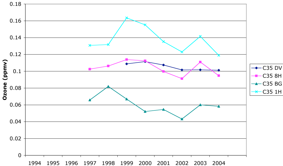
Figure 9: Trends in characteristics of the third- to sixth-highest 8-h ozone events at station C35 (Deer Park).
