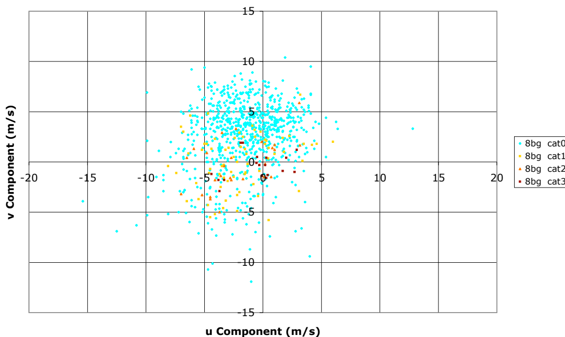
Figure 27: Background ozone concentrations as a function of 24-hour mean resultant buoy winds, May-Sept., 1998-2003. Cat 0: Background ozone less than 0.060 ppmv. Cat 1: Background ozone between 0.060 ppmv and 0.070 ppmv. Cat 2: Background ozone between 0.070 ppmv and 0.080 ppmv. Cat 3: Background ozone greater than 0.080 ppmv.
