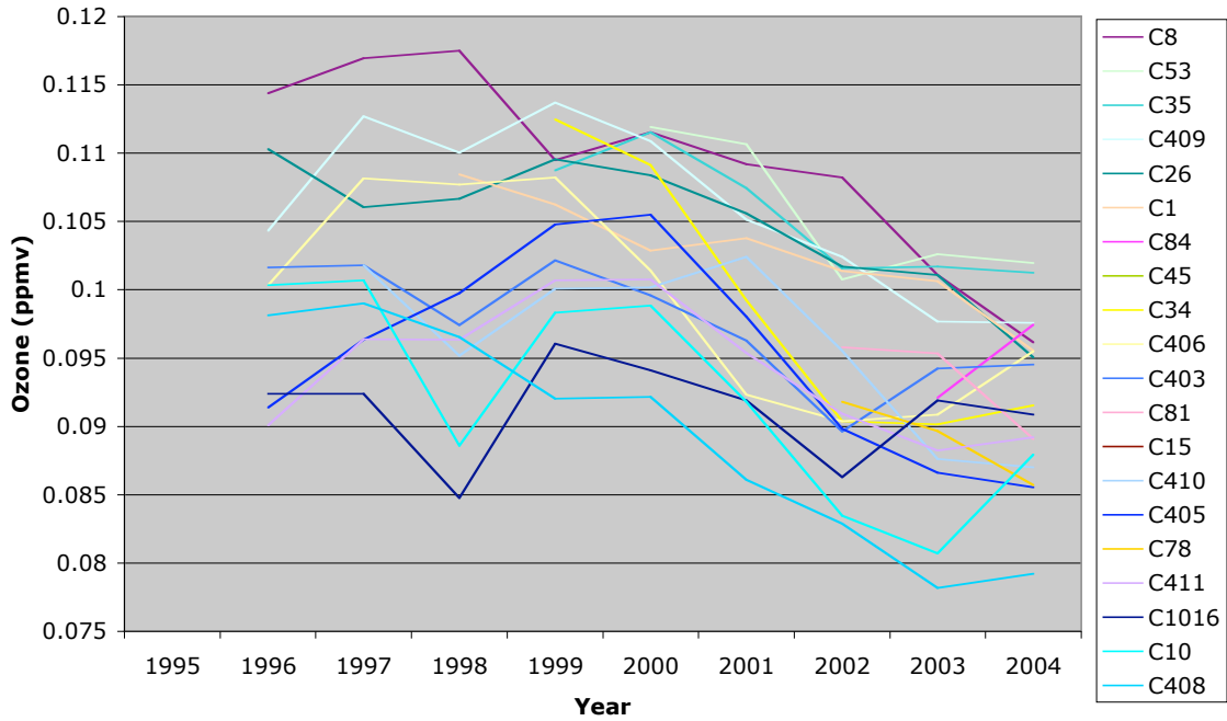
Figure 4: 8-h ozone design values for Houston monitors, computed as the three-year average (labeled with the ending years) of the fourth-highest annual ozone level at each monitor. The legend depicts the monitoring sites in approximate order of design value.
