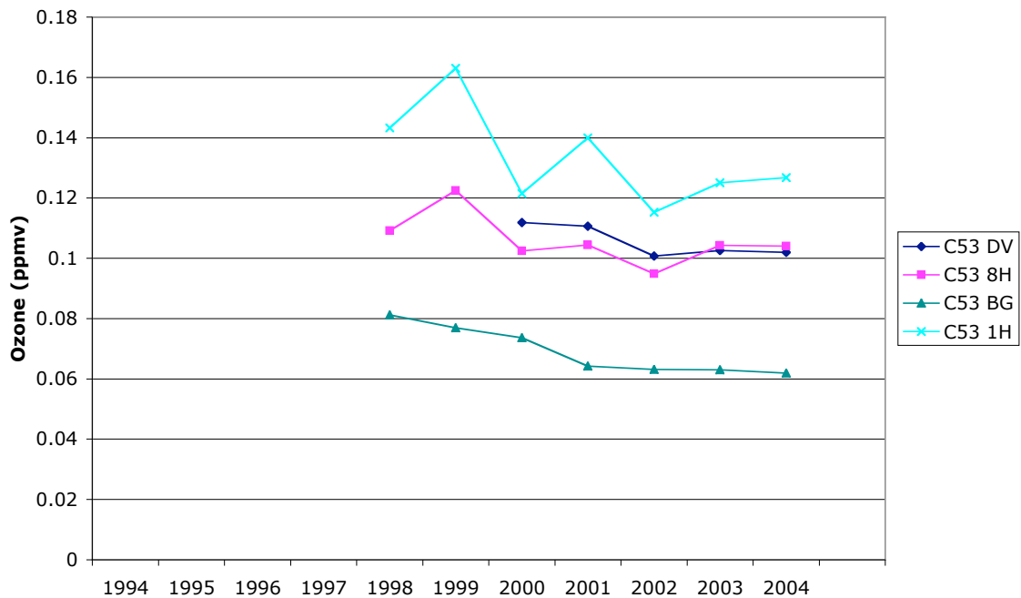
Figure 7: Trends in characteristics of the third- to sixth-highest 8-h ozone events at station C53 (Bayland Park).
