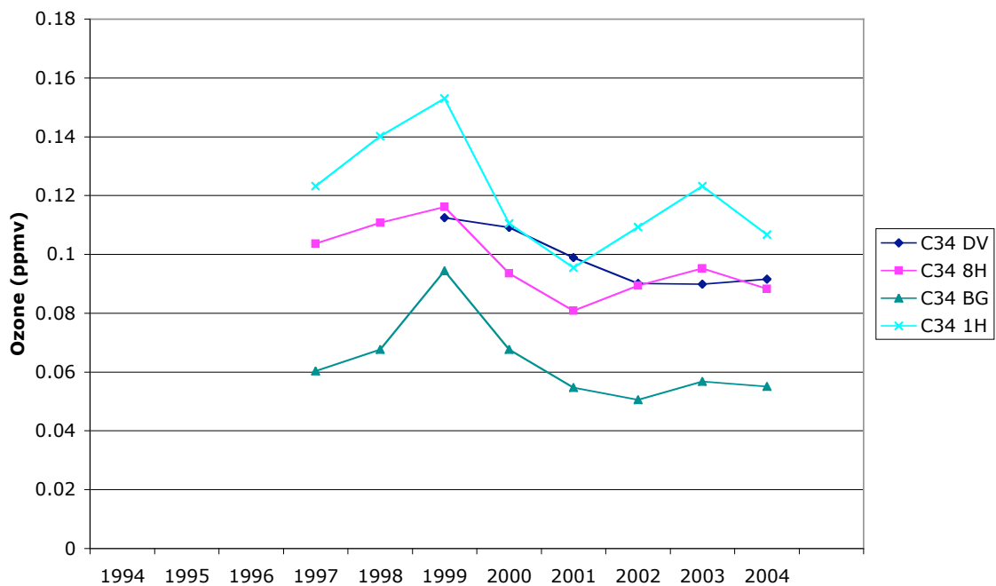
Figure 8: Trends in characteristics of the third- to sixth-highest 8-h ozone events at station C34 (Galveston).
