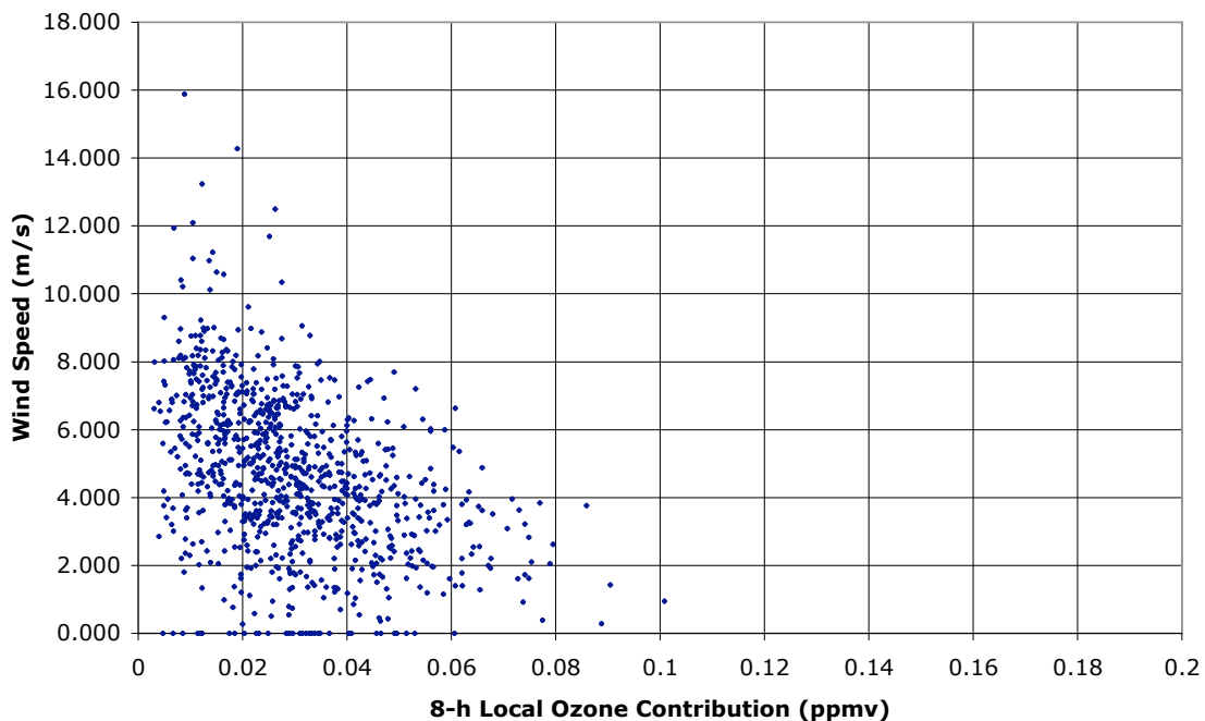
Figure 23: Local contribution to 8-h ozone in Houston and its dependence on mean resultant wind speed, May-Sept., 1998-2003.
