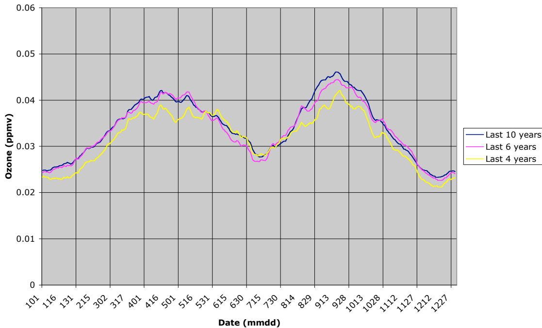
Figure 11: Background 8-h ozone in Houston, averaged over the 10-year period 1994-2003 (blue), the 6-year period 1998-2003 (purple), and the 4-year period 2000-2003 (yellow). A triangular filter was used to smooth the data.
