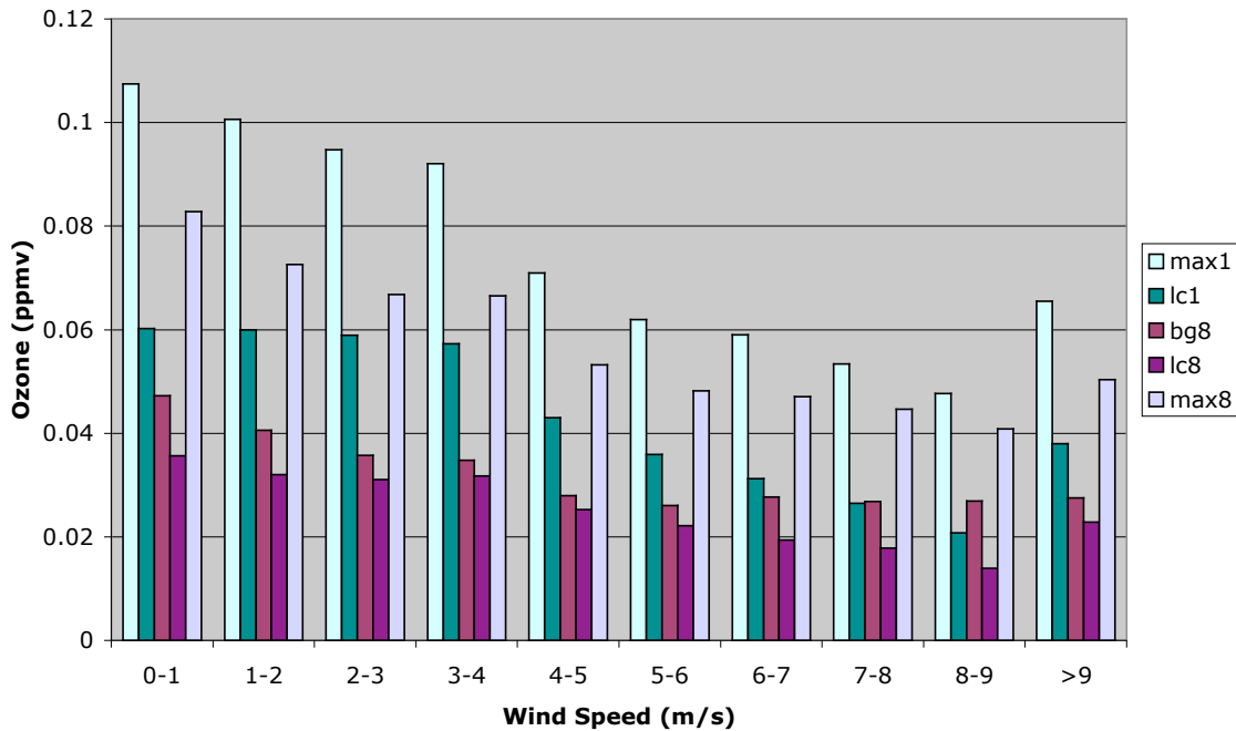
Figure 20: Maximum 1-h ozone, local contribution to 1-h ozone, background ozone, local contribution to 8-h ozone, and maximum 8-h ozone in the Houston region, as a function of resultant vector wind speed at buoy 42035, May-Sept., 1998-2003.
