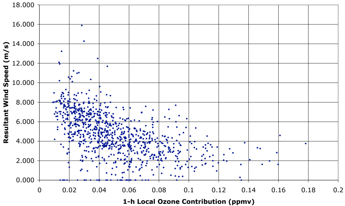
Figure 22: Local contribution to 1-h ozone in Houston and its dependence on mean resultant wind speed, May-Sept., 1998-2003. Points along zero wind speed axis indicate missing wind data.
