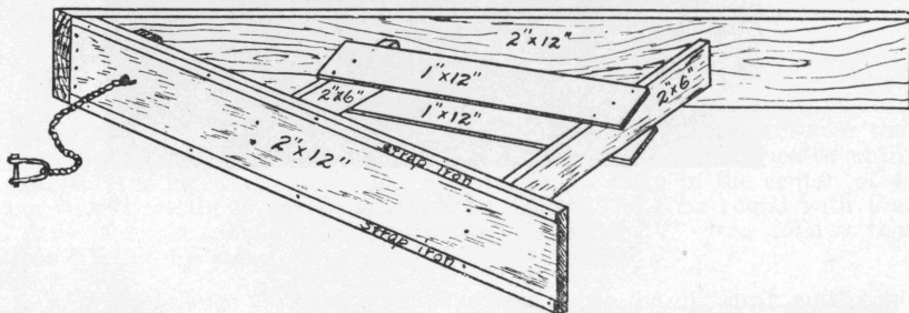
FIG. 8.—Reversible "V" drag.
