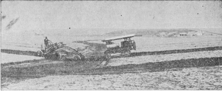
FIG. 9.—County road outfit building a terrace. Shown crossing a gully.
