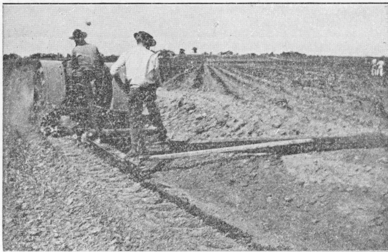
FIG. 13.—Steel ditcher with wooden board extension wing. This extension makes it possible to push dirt to the center of a broad ridge while the tractor runs on solid ground.
