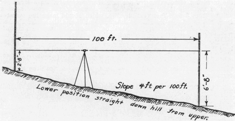
FIG. 2.—Showing how slope of land is measured to obtain a value to use in top line of figures in the "Terracing Table." Slope is measured straight up and down hill, and should be taken where it will be an average, if the hillside slope varies throughout the length of the terrace.
