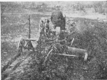
FIG. 11.—Plow terracer. A blade attachment for a gang plow.
