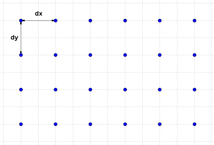
Fig. 14. Rectangular configuration of antenna array elements. Variable dx represents the horizontal element spacing and dy represents the vertical element spacing.
