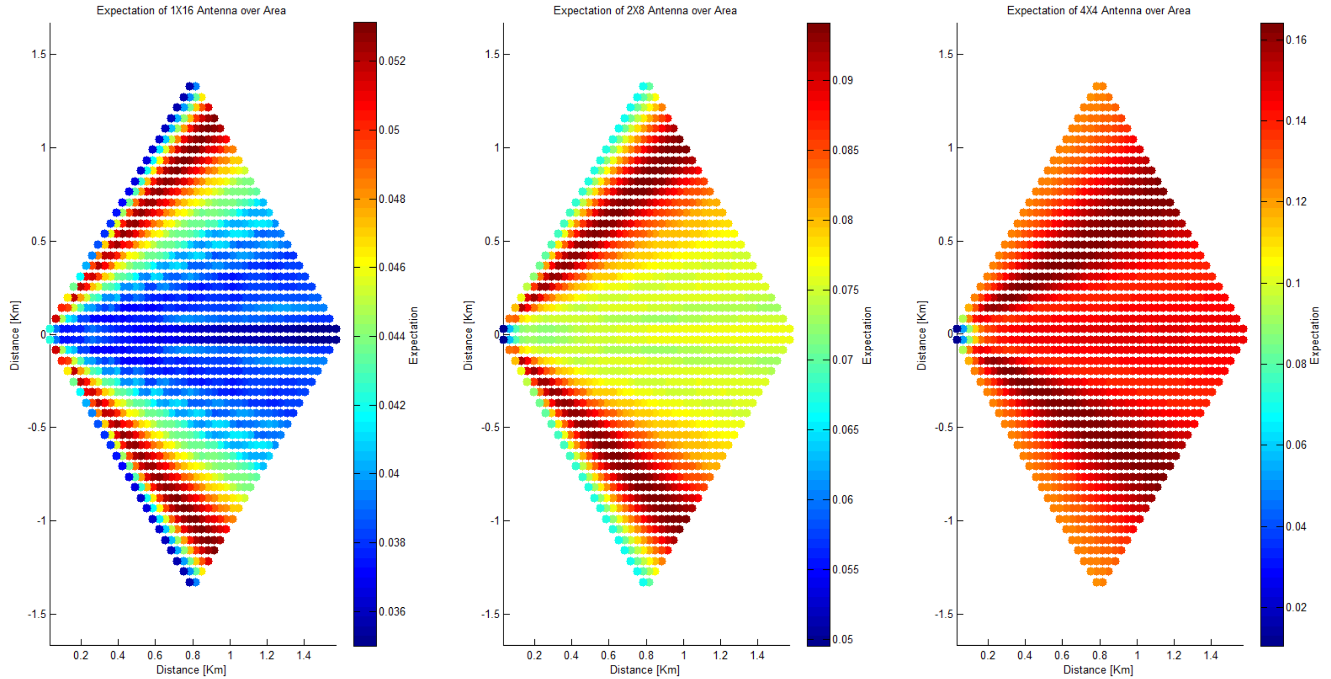
Fig. 32. Uplink Interference Expectation: the expectation of the interference, with distance decay, for each antenna pattern at every grid point (50x50). The expectation was calculated with power taken in units of Watts. The scale of each graph is different based on maximum and minimum expectation values of each. There are 1200 total points within each area.
