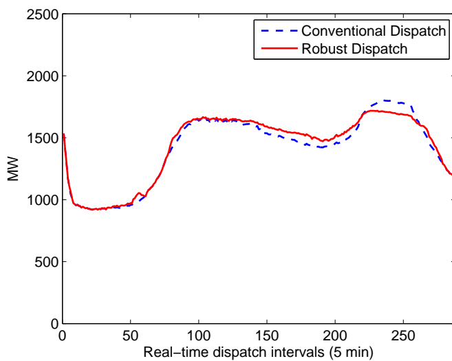
Figure 4.11: System total gas generator profile for entire day
