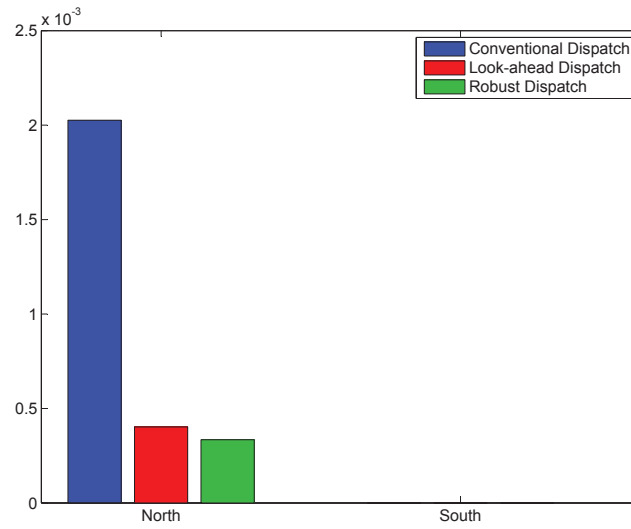
Figure 4.18: Mean LORP comparison for north and south zones
