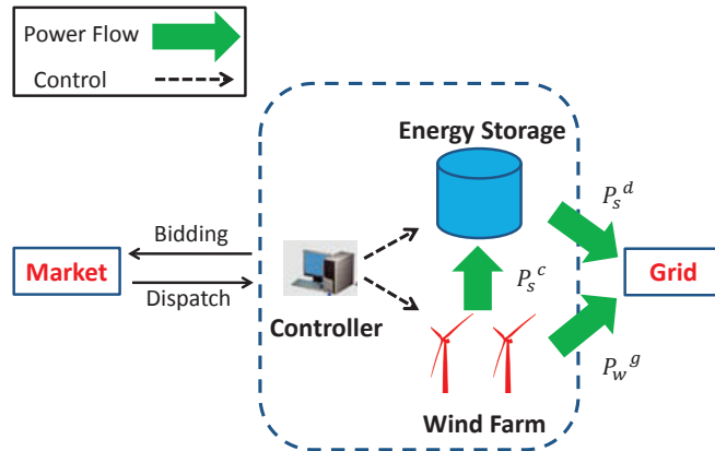
Figure 3.1: Schematic of wind farm and energy storage
