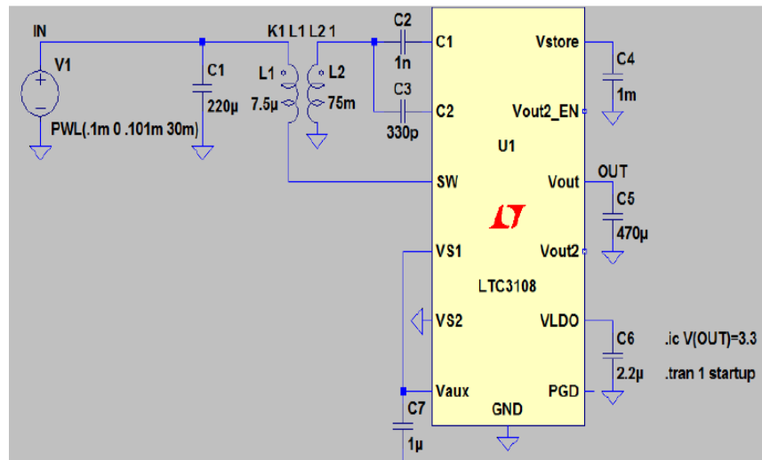
Figure 9: Circuit for Thermal Energy Harvesting
