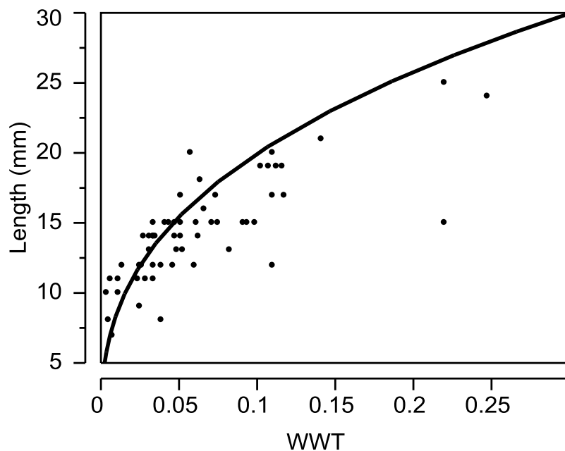
Figure 4.3: Scatter plot of length (mm) and wet weight (g) of oyster spat (n=62) sampled from the study site. The line represents the predicted length (mm) calculated as L=10^{1.67} W_{WWT}^{0.37} .
