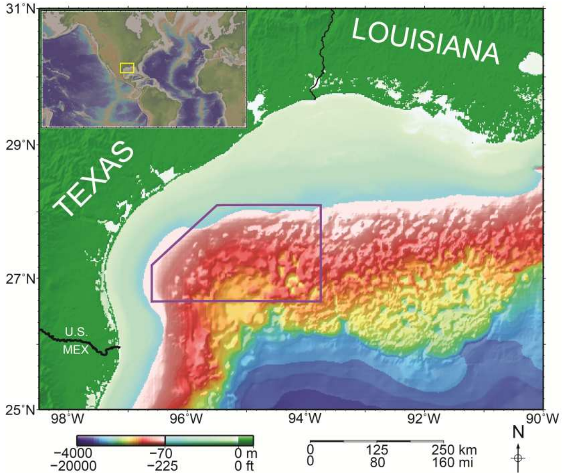
Figure 1: Location and Regional Bathymetry
