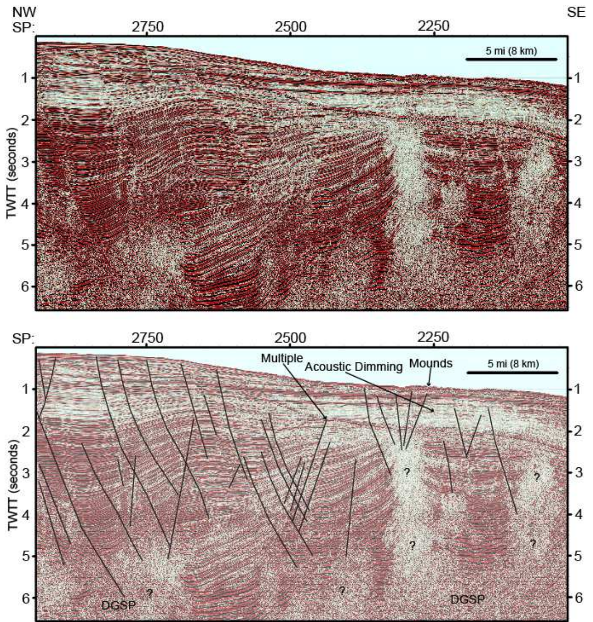
Figure 6: Western Region Faults and DGSP
