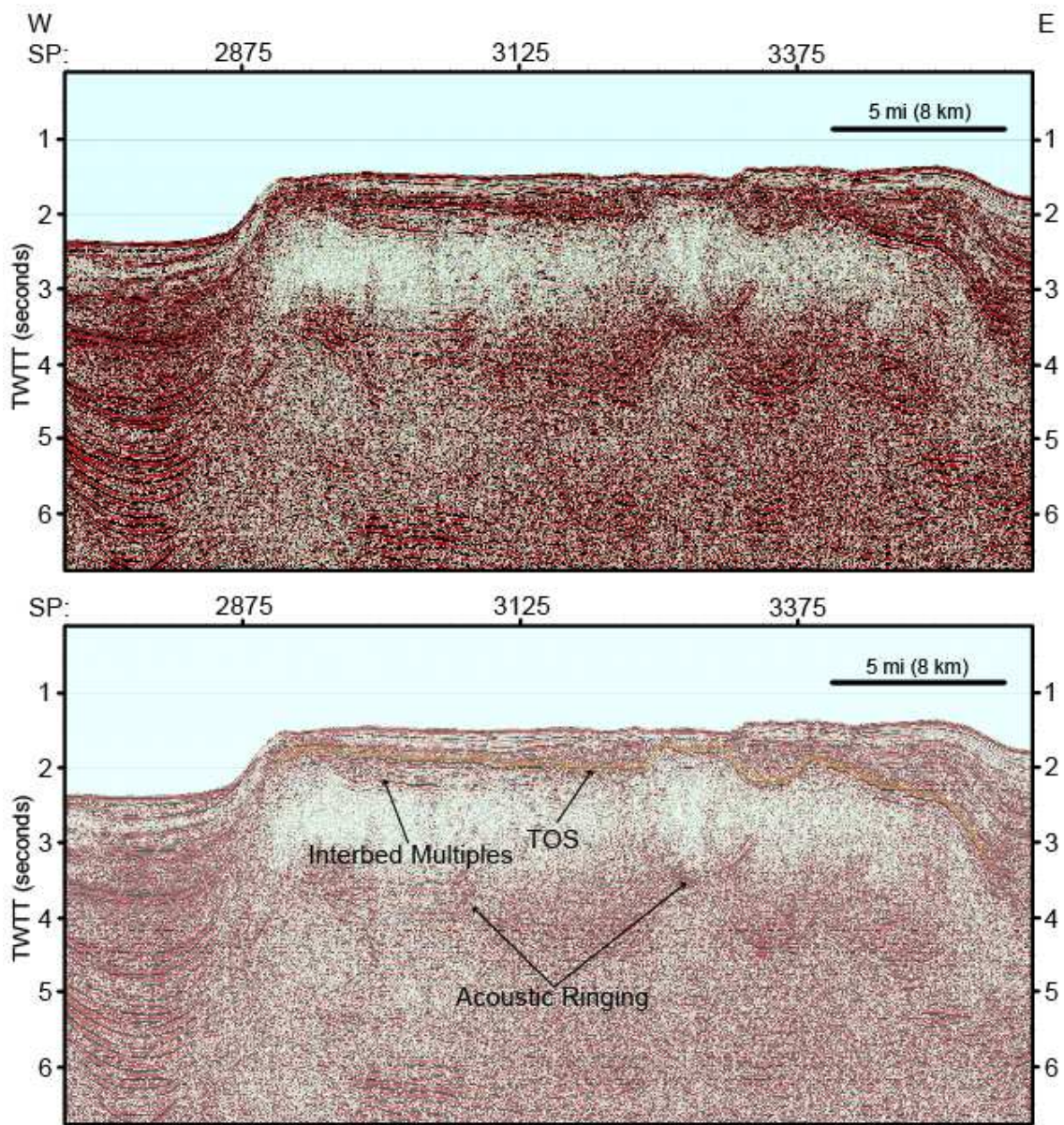
Figure 4: Eastern Region Salt
