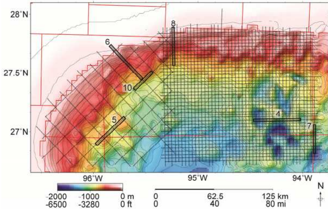
Figure 2: Bathymetry and Seismic Grid
