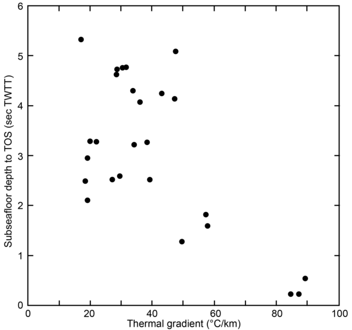
Figure 11: Thermal Gradient Plot
