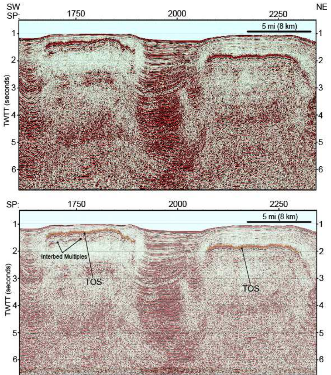
Figure 5: Western Region Salt
