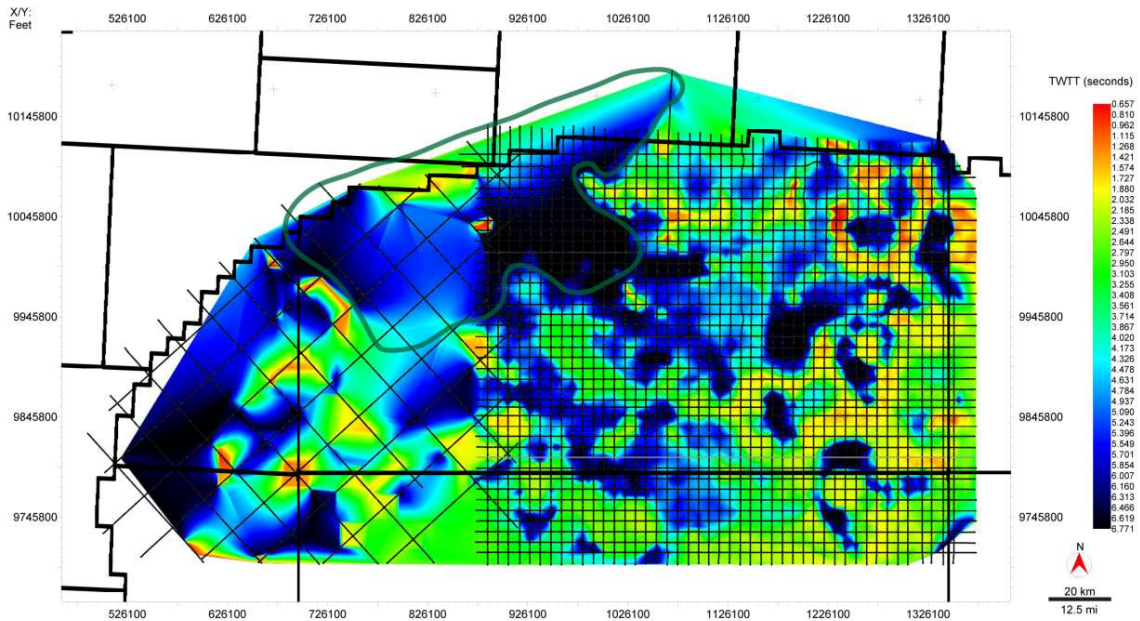
Figure 3: Map of Top of Salt (TOS)
