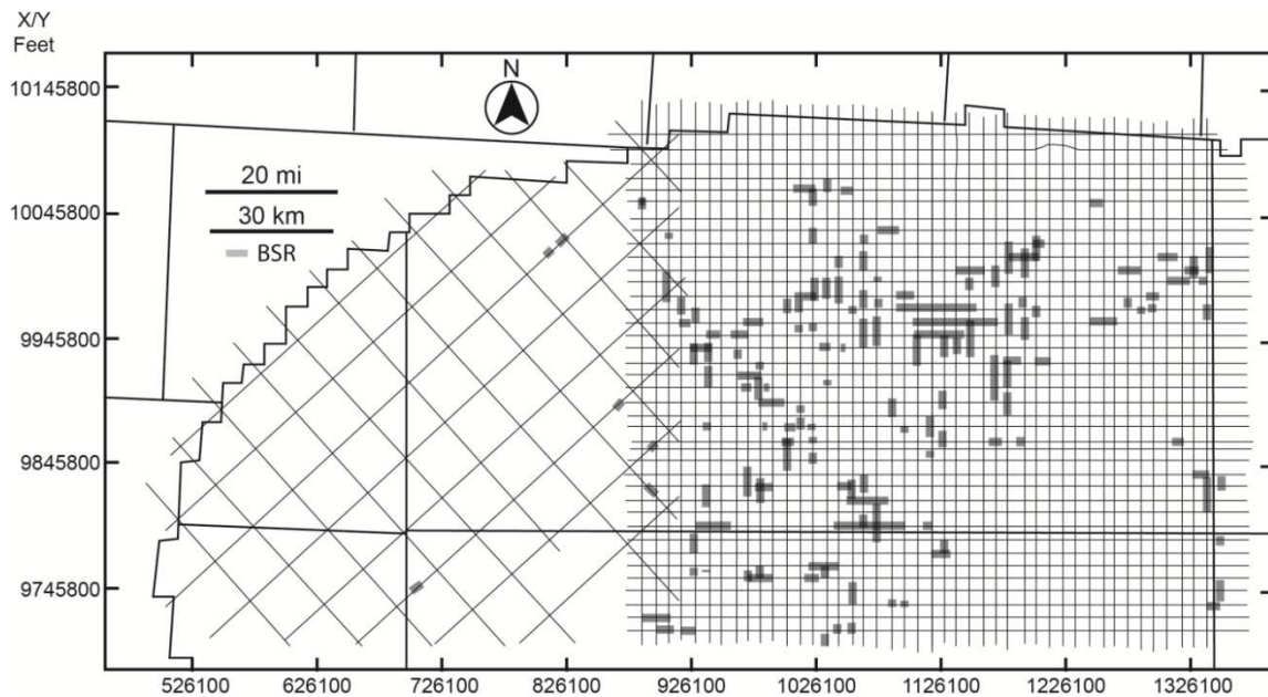
Figure 9: Locations of Interpreted BSRs
