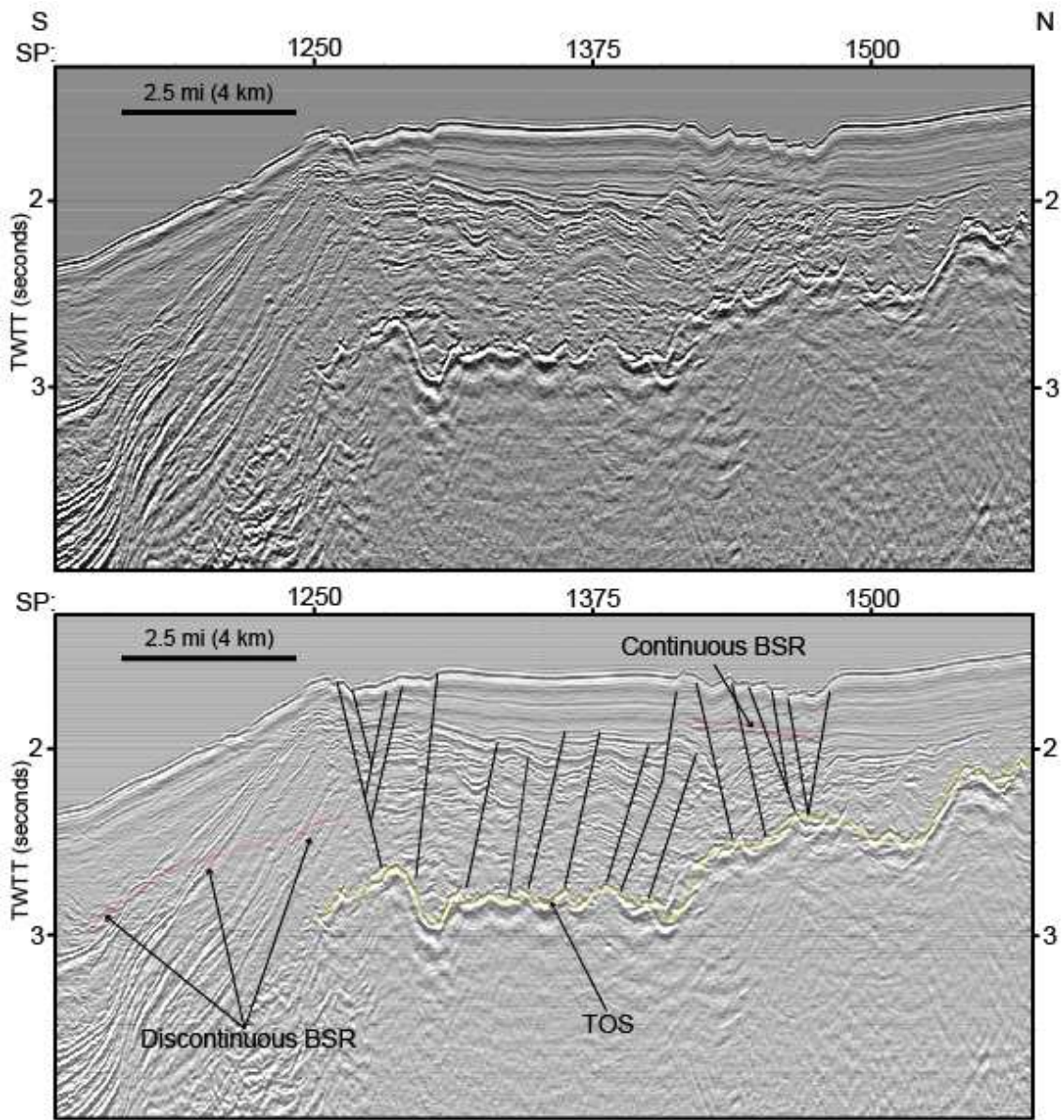
Figure 7: Eastern Region Faults and BSR Examples
