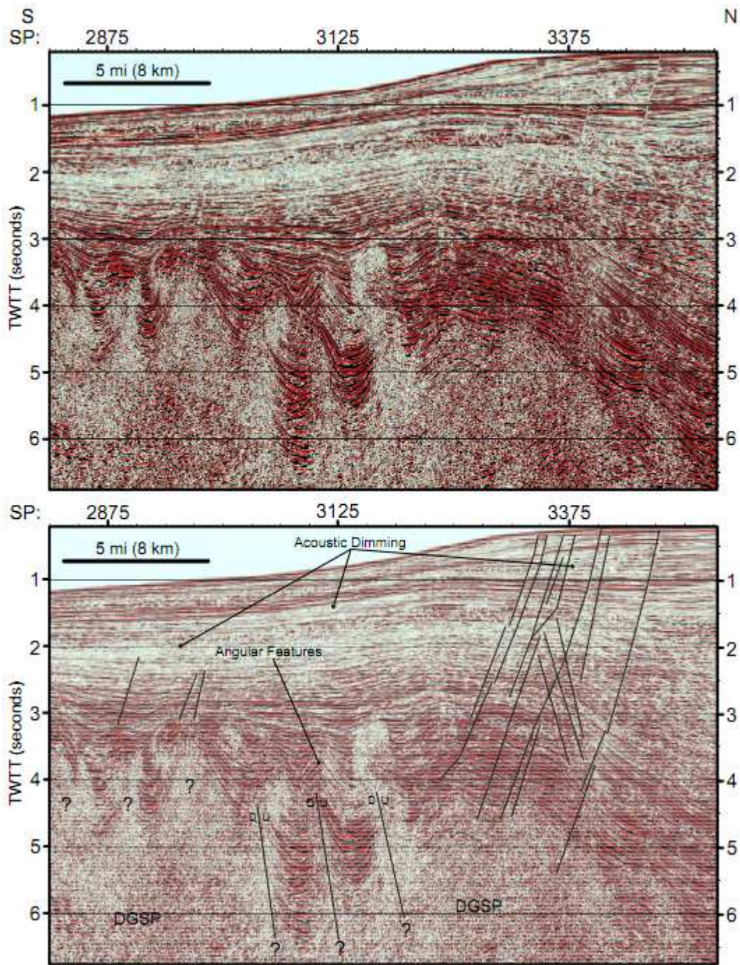
Figure 8: S-N DGSP Seismic Section
