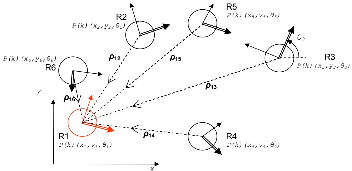
Fig. 4. The problem scenario. There are 6 robots in this example. At this instant, all the robots R2 to R6 are giving pose estimate for R1.
