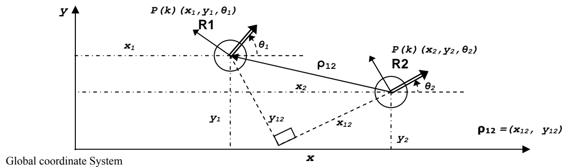
Fig. 1. Pose and range vector. The figure shows the top view of the robots R_1 and R_2 at instant k . Each robot has a coordinate system attached to it.
