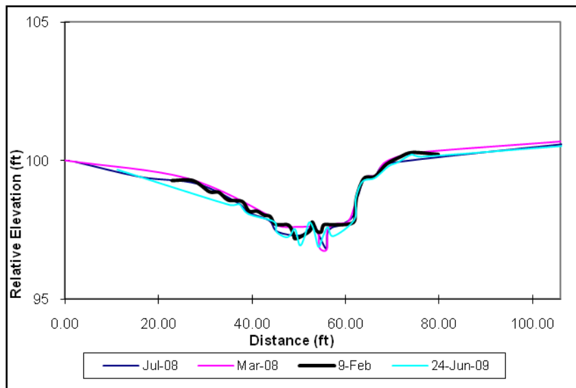
Figure 2. Stream cross sections conducted in 2008 and 2009 on Clear Fork of Plum Creek.
