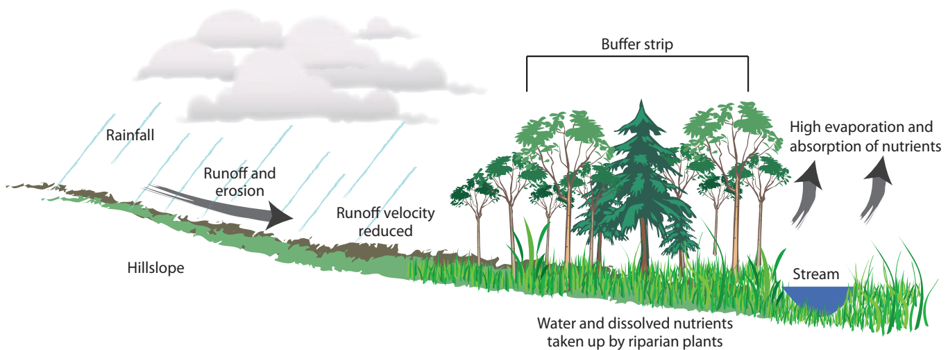
Figure 15. Conceptual model of how vegetated filter strips function to protect the stream from contaminants and the riparian area from erosion. Illustration courtesy of Jennifer Peterson.
