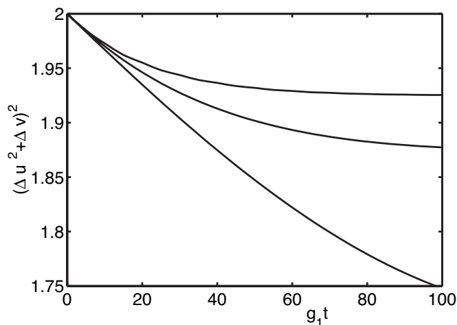
FIG. 4. The quantity (\Delta\hat{u})^2+(\Delta\hat{v})^2 changes with time for several values of the cavity decay rates \kappa . From top to bottom \kappa = 0.02, 0.01, 0 . Other parameters are \Omega=200 , g_1=1 , g_2=2 , and \delta = 1000 .
